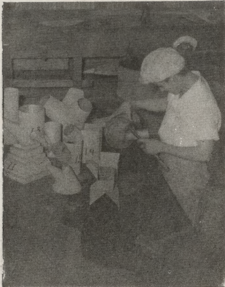
Shown above is Adolpho Oduber of the Tin Shop, with some of the objects he has made under the guidance of Dewie Perkins, Tin Shop supervisor. Mr. Oduber has been in one of the apprentice training classes since 1939, spending two hours daily in classwork, while his job training has consisted in projects of the sort shown in the picture, together with regular shop work.
